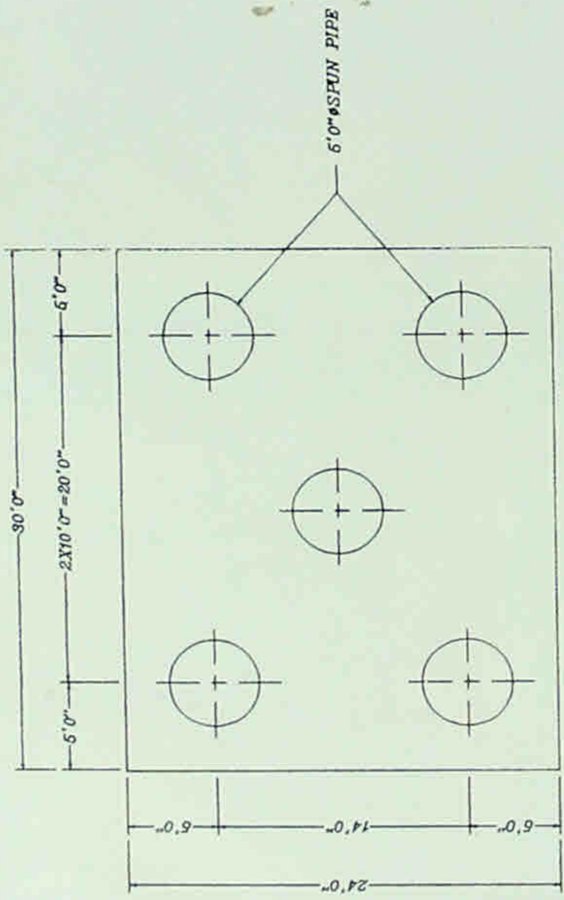
CAP FOUNDATION PLAN
